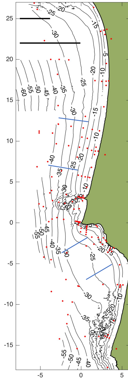
Easting (km)
