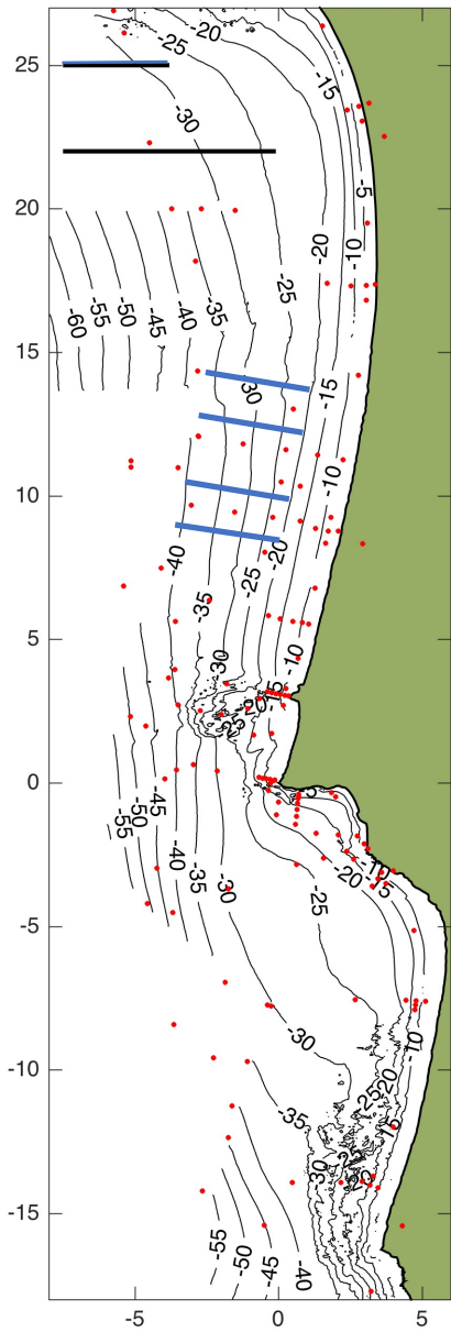
Easting (km)
